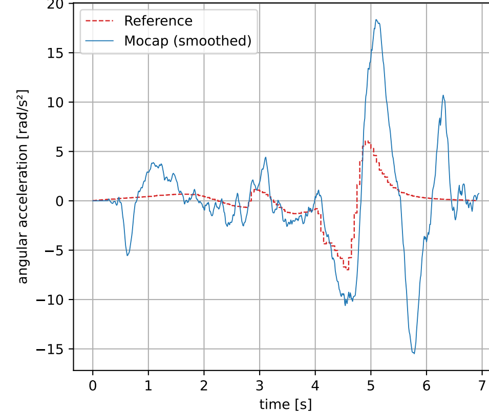
Angular Acceleration
